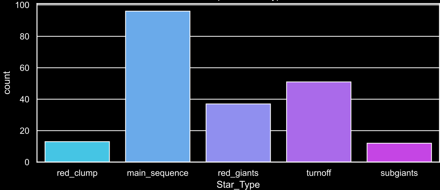
Field [6] Count plot of Star Type
