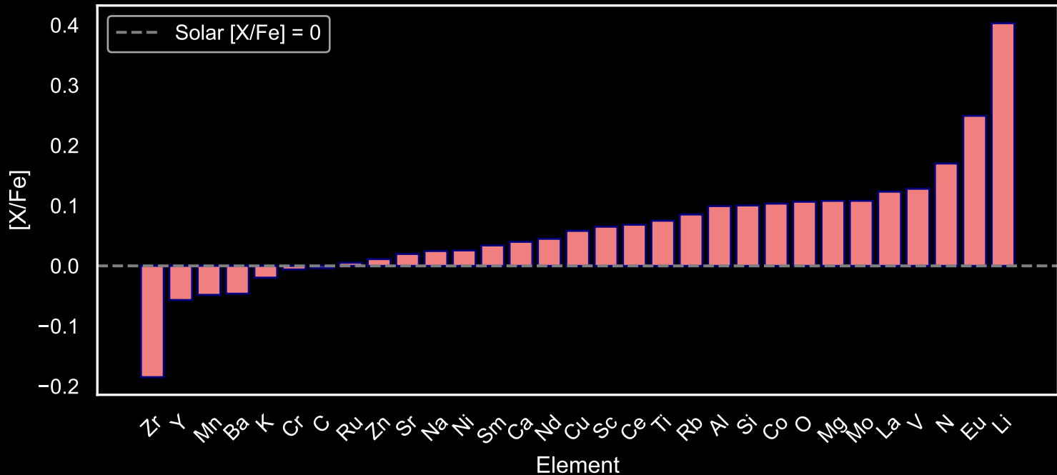
Abundance Pattern for GALAH Star Field [6] (N=209)
