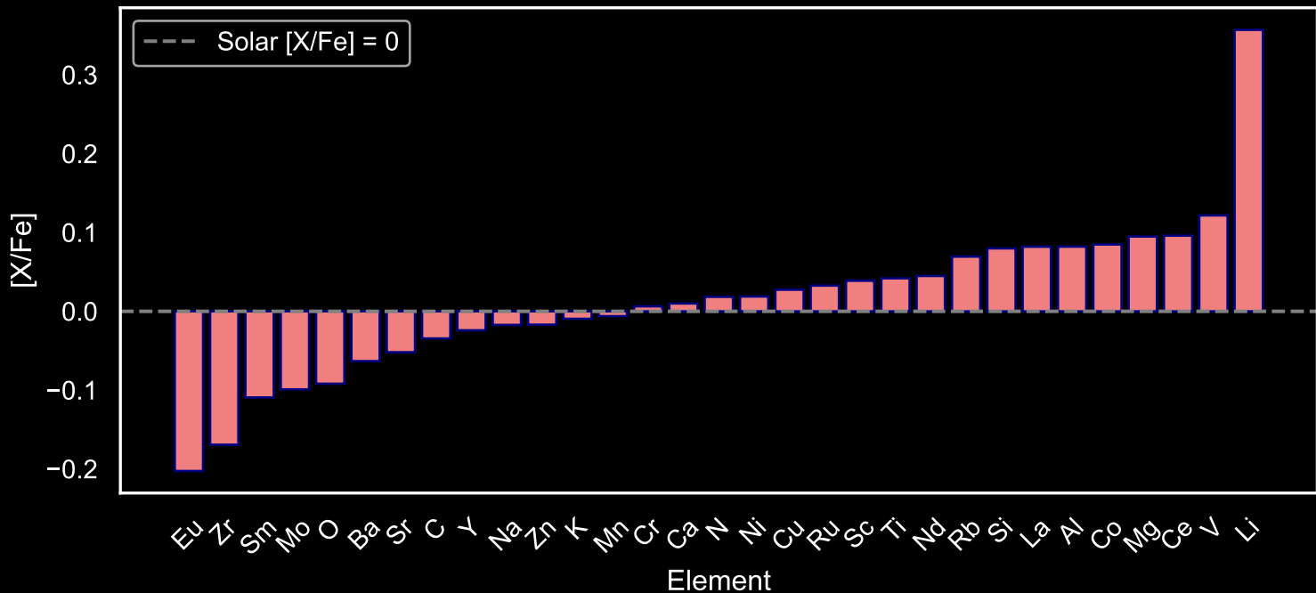
Abundance Pattern for GALAH Main Sequence Stars: Star Field [6] (N=96)
