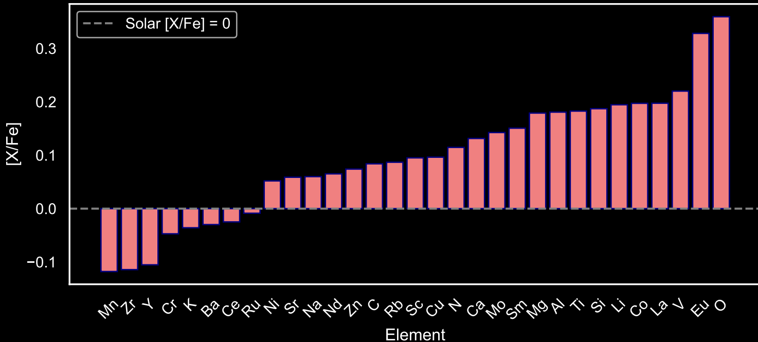
Abundance Pattern for GALAH Red Giants: Star Field [6] (N=50)
