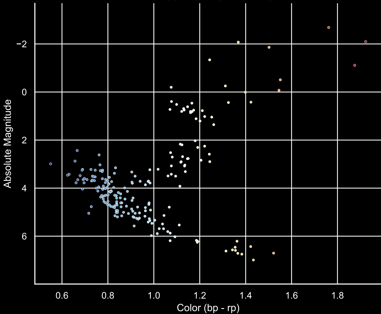
GALAH Hertzsprung-Russel Diagram Field [6] Ra [327.3] Dec [-21.98]
